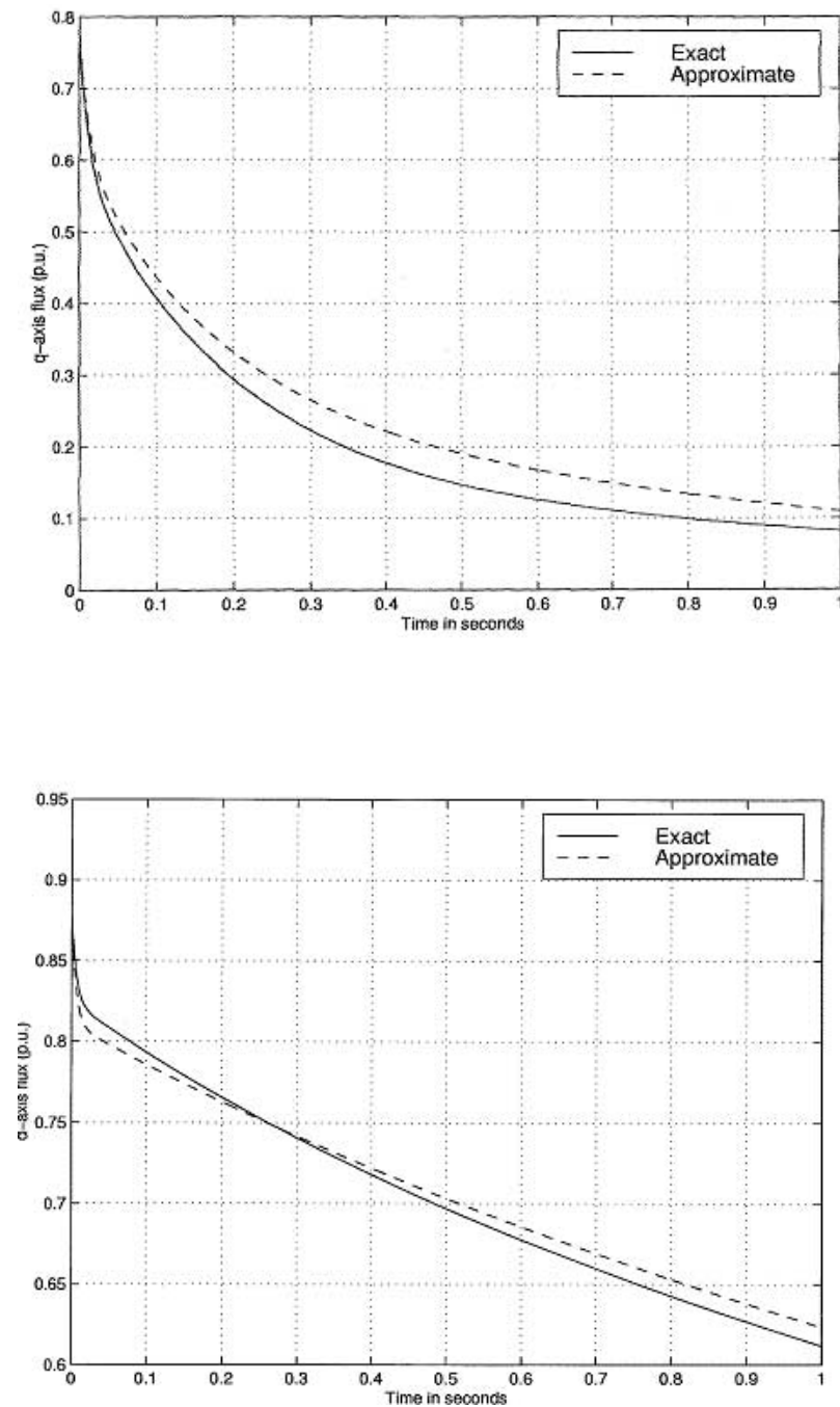
Figure 18—Assessment of numerical (exact) and closed-form (approximate) computations of time constants and related quantities
