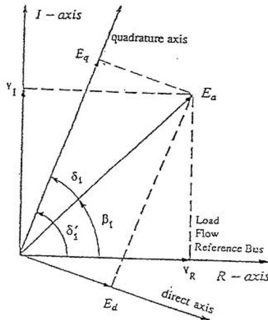
Figure 3—Relationship between d and q axes and real and imaginary axes
