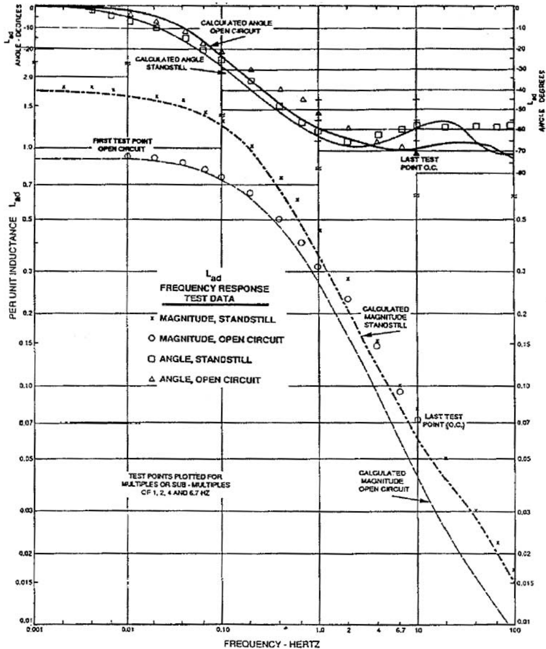
Figure 10—Comparison of the d-axis armature field mutual inductance, L_{ad} at open circuit rated voltage and at standstill: test data and finite-element calculated data
